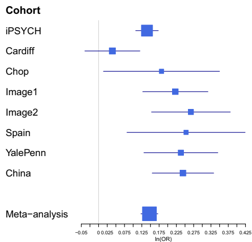
Fig. 2 Forest plot for the index variant (rs7118422) in the genome-wide significant locus on chromosome 11. Forest plot for the effect size estimates (natural logarithm of the odds ratio (ln(OR))) in each included cohort, estimated from logistic regression, and in the trans-ancestry GWAS meta-analysis of European and Chinese cohorts (4208 cases and 32,222 controls) using an inverse-variance weighted fixed effects model. In addition, standard errors of the ln(OR) estimates. For information on sample sizes, allele frequencies and P -values for rs7118422 in the single cohorts see Supplementary Data 1.
