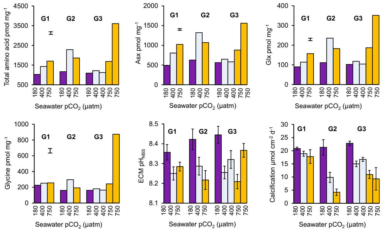
Figure 1. Skeletal amino acid concentrations of each coral genotype (G1, G2 and G3) cultured at 25 °C and over a range of seawater pCO 2 . Two replicate colonies of G3 were cultured at 400 and 750 µatm. Error bars indicate the mean standard deviation of analyses of duplicate drilled samples. Calcification rates 20 (error bar shows typical standard deviation of 3–4 measurements per colony) and calcification site pH 21 (adjusted to the pH NBS scale, error bars show 95% confidence limits) are shown for reference. Asx aspartic acid + asparagine, Glx glutamic acid + glutamine.
