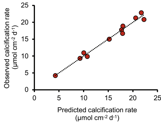
Figure 3. Observed and predicted coral calcification rates. Predicted rates were modelled using a multiple linear regression model of concentrations of Asx, Glx, serine, alanine and total amino acid and pH_{ECM} .
