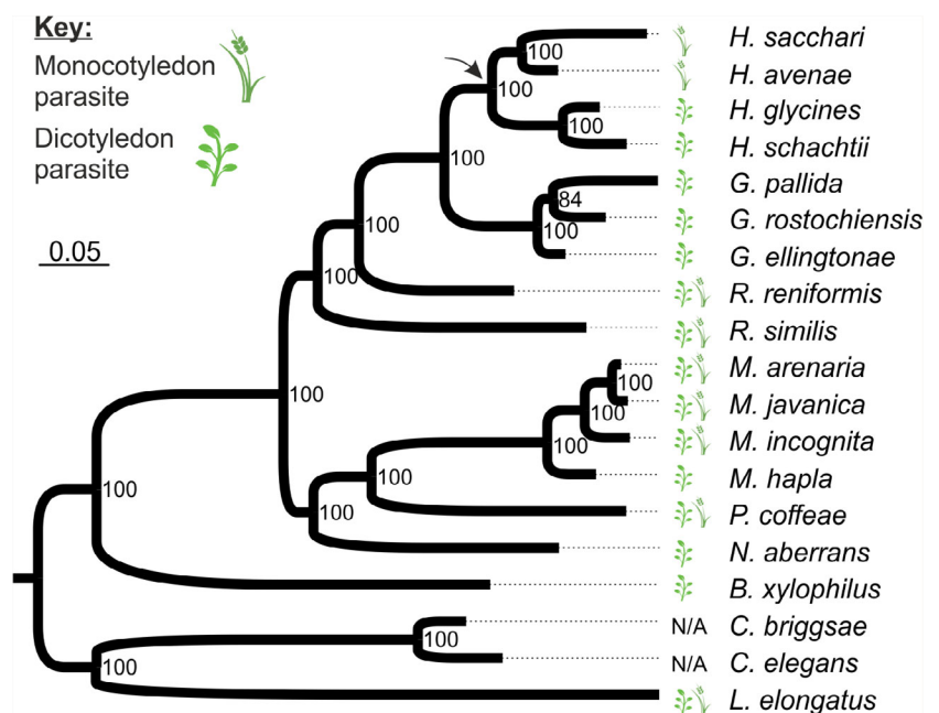
Figure 1. Phylogenetic analysis of 96 CEGMA genes conserved in 19 species of nematode shows that H. sacchari and H. avenae share a common monocot-parasitic ancestor that most likely evolved from a parasite of dicots (indicated by the arrow). The scale bar indicates substitutions per base. Node labels indicate support values for 1000 bootstraps.
