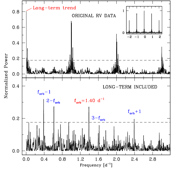
Fig. 3. ISW power spectra of the HARPS-N radial velocity data. The horizontal line marks FAP=1%. Top panel: the long-term trend is the main feature in the original data. The insert shows the spectral window of the data. Bottom panel: the orbital frequency of HD 80653 b is clearly detected when a quadratic trend is added as a known constituent.
