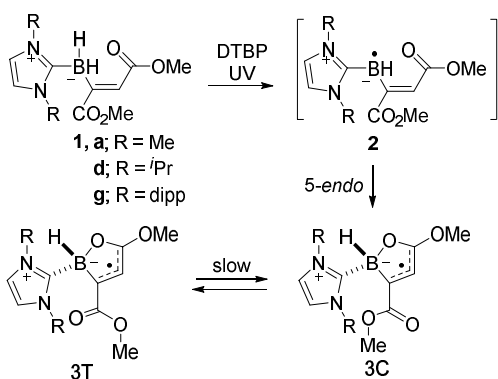
Scheme 3. Generation of NHC-oxaborole radicals with methyl ester substituents.
