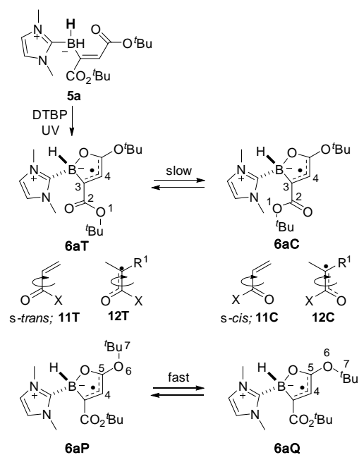
Scheme 2. Conformational interconversions of 1,2-oxaborole radicals 6a . Top: CO 2 t Bu rotor; bottom: O t Bu rotor.
