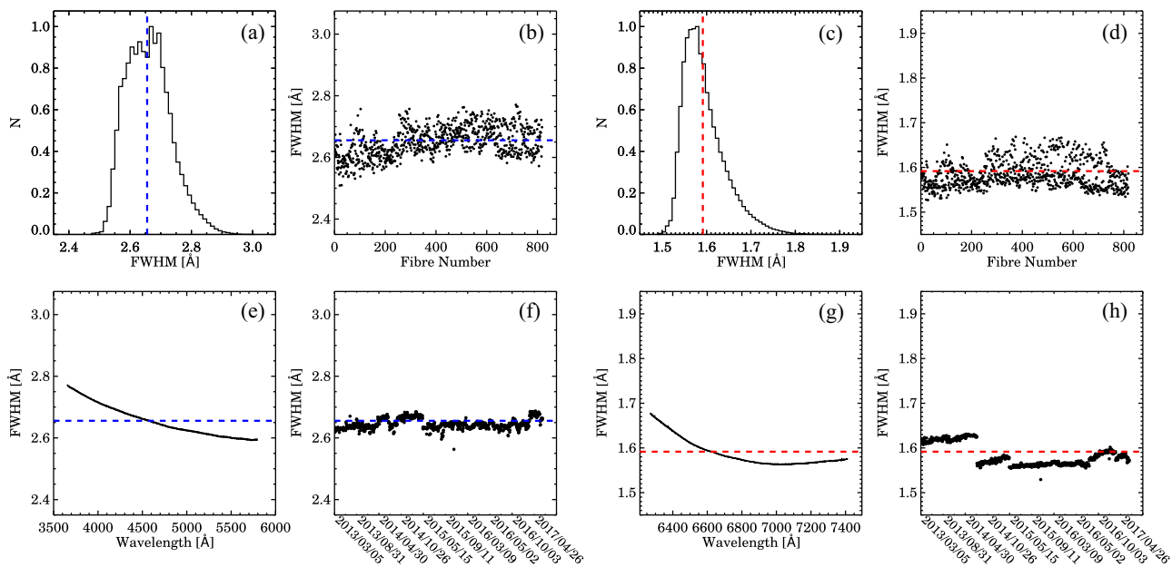
Figure 2. SAMI-AAOmega spectral resolution in the blue arm and the red arm derived from reduced arc-line frames. Panels a, b, e, and f show the FWHM distribution, FWHM versus fibre number, FWHM versus wavelength, and FWHM versus date in the blue data (note that dates are linearly spaced on frame number, not time), and similar for panels c, d, g, and h for the red data.
