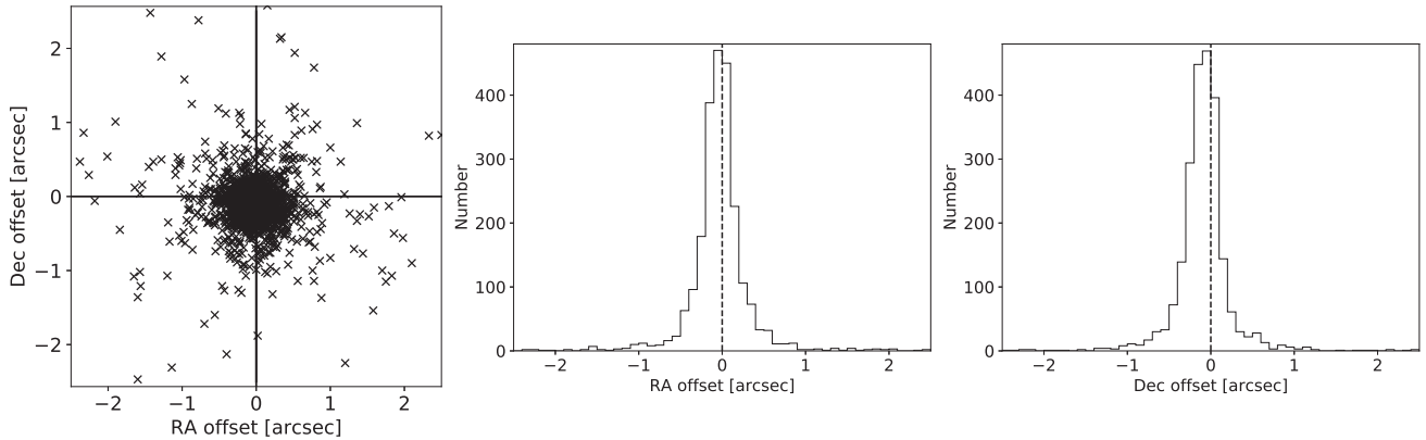
Figure 6. Offset between the SAMI cube WCS and KiDS r -band imaging. The left-hand panel shows the offsets for all DR2 galaxies. Note that 24 galaxies with large offsets lie outside the figure. The centre and right-hand panel show histograms of the offset in RA and Dec., respectively. Catastrophic failures have not been removed.
