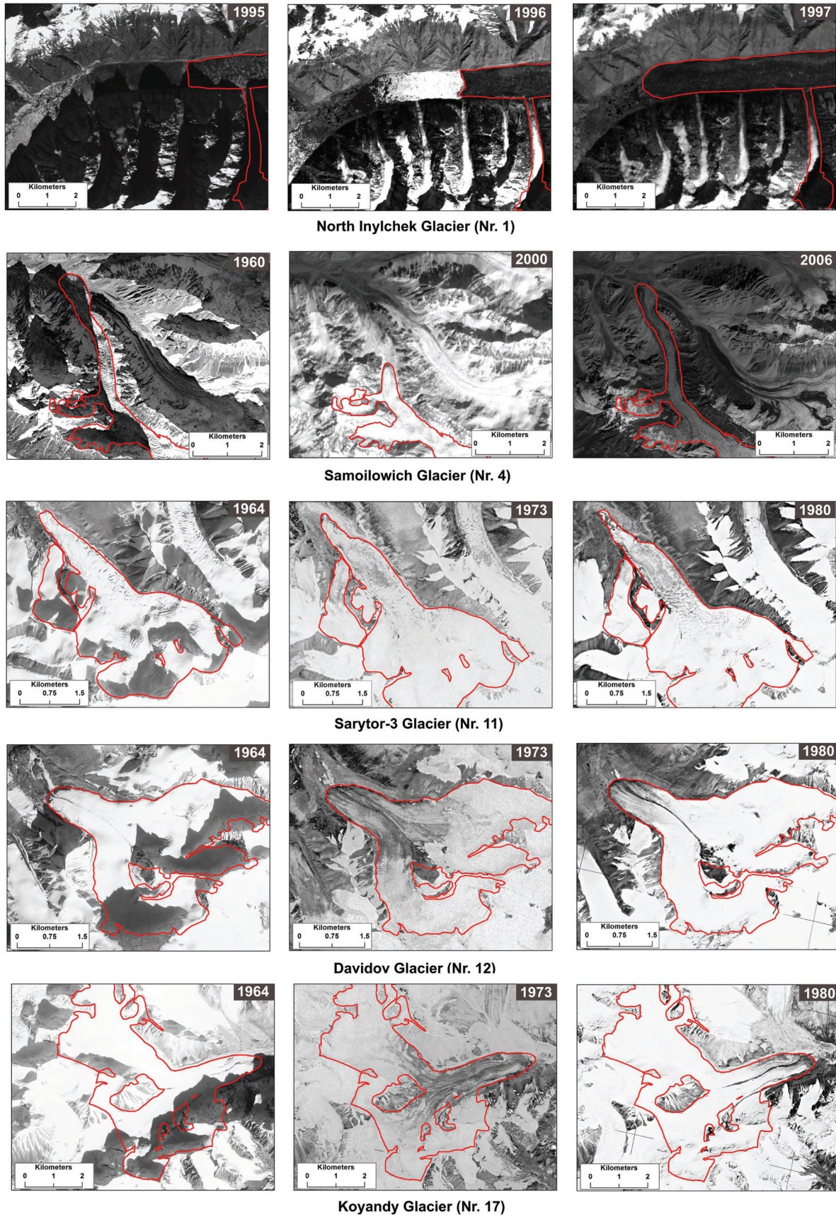
FIGURE A1. Surge in some glaciers of central Tien Shan and Ak-Shirak.
