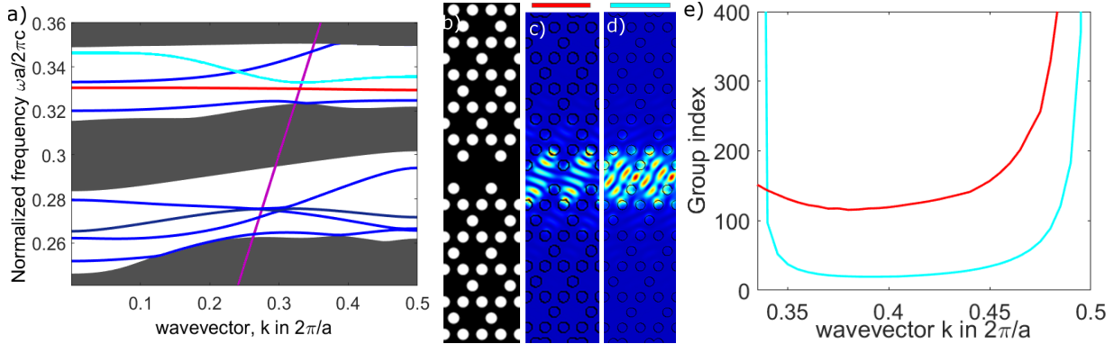
Figure 3: (Colour online) a) Dispersion curve of the waveguide under investigation. The modes of interest, lying in the second bandgap, are highlighted in red and light blue. The light line is shown in purple. b) Sketch of a section of the kagome-lattice waveguide. The waveguide width is conventionally given as wa\sqrt{3} , as indicated in the sketch. In our case w = 0.8 and a = 500 nm. c) and d) representative field distributions of the optical modes shown in a) as red and light blue, respectively, plotted for k = 0.4 . The field profiles differ significantly from that of a traditional triangular-lattice waveguide and indicate an intermediate behaviour, between a traditional waveguide and a cavity based system, providing an intuitive understanding of the origin of the slow light in this waveguide. e) Group index of the two waveguide modes plotted against wavevector. Only the guided mode region, below the lightline, is shown. The two modes have a minimum group index of 20 and 125 respectively.
