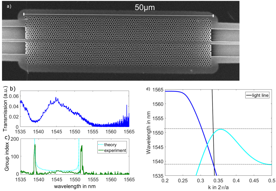
Figure 4: (Colour online) a) Scanning electron microscope image of an air-bridge kagome-lattice PhC waveguide. b) Experimental transmission spectrum of the waveguide shown in a). c) Experimental (solid, green) and theoretical (dashed, light blue) group index spectra. The corresponding bandstructure is shown in d). The solid black line indicates the light line and the dark blue line an additional mode that co-exist in the observed wavelength region. The stationary points in the bandstructure occur at the same wavelength as the peaks in the group index spectra (indicated by the black dashed lines). Therefore, both the experimental and theoretical group index are limited by the measurement/simulation resolution and the high group index peaks are associated with stopped light, which is occurring below the light line and - for the high wavelength peak - away from the bandedge ( k = 0.36 ).
