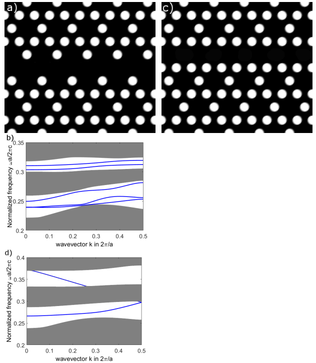
Figure 2: (Colour online) Sketch of different waveguides in a kagome lattice and their respective bandstructure. a) is formed by removing a complete row, with the bandstructure shown in b). c) is formed by removing a sparse row and the corresponding bandstructure is shown in d). In the bandstructure plots blue indicates a waveguide mode, white indicates the photonic band gap regions and grey shading indicates bulk modes.
