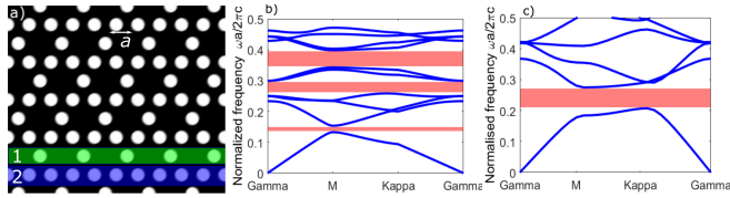
Figure 1: (Colour online) a) Sketch of a kagome lattice of low-index holes in a high-index background. 1 indicates a sparse row, where every second lattice site is missing and 2 indicates a complete row, identical to that of a triangular lattice with the same hole spacing, a . b) Simulated bandstructure of the kagome lattice for TE polarized light. c) Bandstructure of a triangular lattice (TE polarized light) for comparison. In both b and c the shaded regions indicate the photonic bandgaps.
