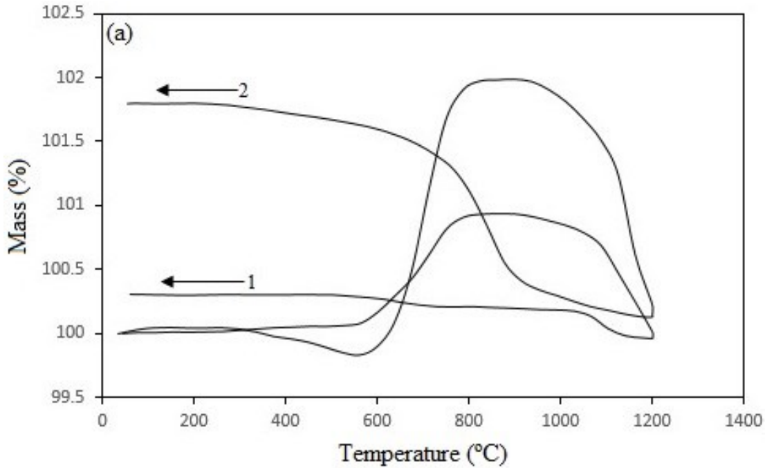
Fig. 5 (a) Thermogravimetric analysis of (1) Ba 0.5 Sr 0.5 Ce 0.6 Zr 0.2 Gd 0.1 Y 0.1 O 3- \delta and (2) BaZr 0.3 Ce 0.5 Y 0.1 Yb 0.1 O 3- \delta heated up to 1200 °C in pure CO 2 with a flow rate of 40 ml/min and with a heating/cooling rate of 3 °C/min.
