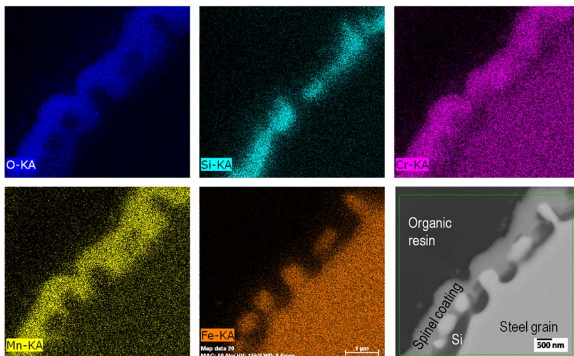
Figure 6 EDX maps collected at the interface spinel/MS for a Mn-infiltrated 1% 3YSZ-MS.
