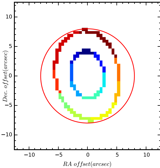
Figure 4. An example of Annular-Voronoi binning which has been applied to the SAMI data cubes. In this example, spaxels in two annuli with an ellipticity of 0.28 at a position angle of 98^{\circ}.8 and a width of one spaxel are grouped into contiguous subbins, represented here as groups of pixels with the same colour. Spectral fitting, emission line integration and dust corrections are performed independently within each subbin. The red circle represents the size of the SAMI aperture. For clarity, only two annular bins are shown, although the entire SAMI field is partitioned into bins.
