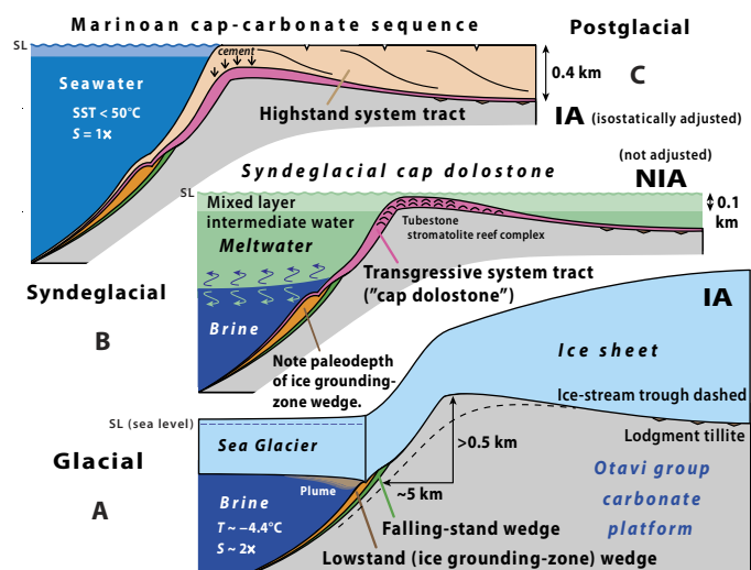
Fig. 26. Three-stage paleoceanographic model for Marinoan cap-carbonate sequences. (A) During the Snowball cryochron, net base-level fall (glacial eustasy > glacial isostasy + ice gravity) causes falling-stand and ice grounding-zone wedges to form on the continental slope, whereas lodgment till is deposited locally above sea level. Salinity of seawater may double, as a result of freshwater sequestration in ice sheets and sea glacier, and the freezing point is lowered accordingly. Glacial action supplies carbonate eroded from the platform to the ocean as suspended load in meltwater plume and grounding-zone wedge. (B) During deglaciation, meltwater production and surface warming create stable density stratification (387). The kilometer-thick meltwater lid (Glacial Lake Harland) includes an oxygenated mixed layer and intermediate water that is at least regionally anoxic, presumably due to respiration of surface organic export production. Marinoan cap dolostone was deposited diachronously from the meltwater mixed layer as base level rose and the glacierized landscape was flooded. The time scale for base-level rise may exceed the ice-sheet melting time scale because of whole-ocean warming and thermal expansion as destratification occurs (387) and over the peripheral bulges of former ice sheets, which collapse on the time scale of isostatic adjustment (IA) (419). (C) After ice sheets have melted, the meltwater lid mixes with the chemically evolved Snowball brine, which finally warms (387). The HST of cap-carbonate sequences fills in areas where net accommodation remains after GIA and hydro-isostatic adjustments. Landward progradation is inferred from inclined surfaces of constant carbonate \delta^{13}\text{C} (97).
