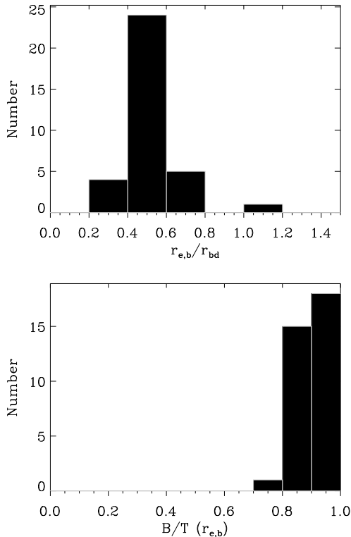
Figure 10. Upper panel. Distribution of r_{e,b}/r_{bd} for our S0 galaxies. r_{bd} represents the radius where the bulge light dominates the SB distribution over any other structural component. Bottom panel. Distribution of B/T ratio computed at one r_{e,b} of the bulge.
