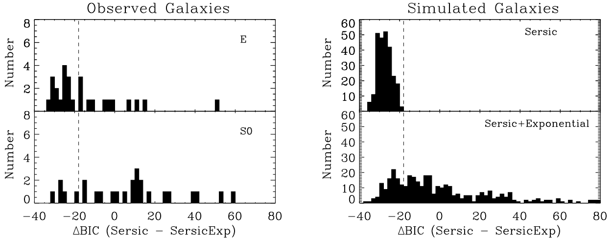
Figure 4. Distribution of \Delta BIC values, BIC(\text{Sérsic}) - BIC(\text{Sérsic}+\text{Exp}) , for our observed galaxy sample (left) and a set of simulated galaxies (right). The upper and lower panels for our galaxy sample represent galaxies visually classified as elliptical (E) and lenticular (S0), respectively. The upper and lower panels for the simulated galaxies represent the single component Sérsic galaxies and the two component Sérsic + Exponential galaxies, respectively. The vertical dashed lines in all panels show the limiting \Delta BIC = -18 for a galaxy considered to be a S0.
