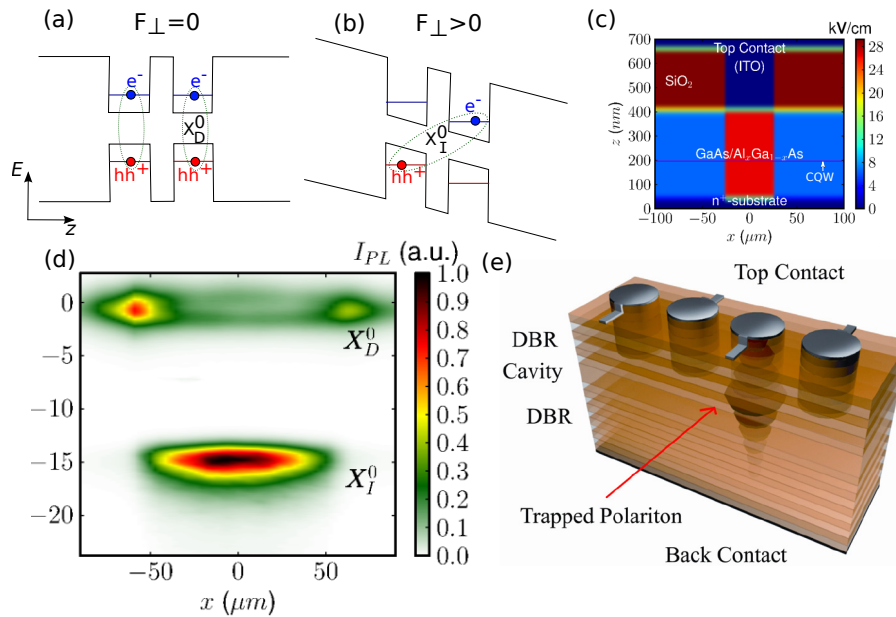
Figure 8. Electrostatic trapping of excitons and exciton-polaritons: (a) and (b) The exciton radiative transition without and with an applied voltage, the latter with long-lifetime indirect excitons X_I . (c) A cross-section of a trap design showing a modulation of the electric field strength felt by the excitons due to shielding by an \text{SiO}_2 layer, and (d) the experimental realization of indirect exciton trapping. These figures are reproduced from [80]. Copyright (2011) by The American Physical Society. (e) Proposed trap for microcavity exciton-polaritons: The microcavity is locally capped by a semitransparent contact which simultaneously acts as a gate. Once a small bias is applied, the polariton energy is lowered underneath the trap, and an attractive potential is created. The figure is reproduced with permission from [89]
