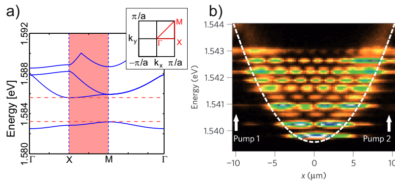
Figure 4. (a) The first four energy bands for a square lattice array of polariton traps in the reduced Brillouin Zone (BZ) representation. Dashed lines indicate the position of the complete band gap. Inset: The first irreducible BZ. (b) Harmonic energy spectrum of a polariton condensate trapped between two laser spots. This figure is reproduced with permission from [66].
