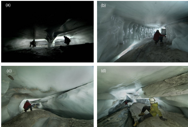
Figure 5. Passage morphology in NG-04. (a) Cut-off meander loop; note the inclined debris band on back wall behind the left-hand person. (b) The upper passage near A12, showing suture between the right-hand wall and the ceiling, and the incised lower passage on the left. (c) The upper passage near A7, with a void and suture between the right-hand wall and the ceiling. (d) The upper passage near A6, showing a band of bedded sand filling a sub-horizontal suture above the foreground person.
