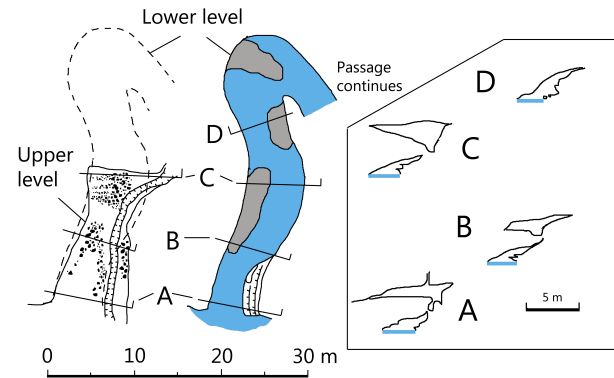
Figure 6. Plan and passage cross sections of conduit NG-05. The plan view of the upper level shows boulders and an incised channel on the conduit floor. For location see Fig. 3a.
