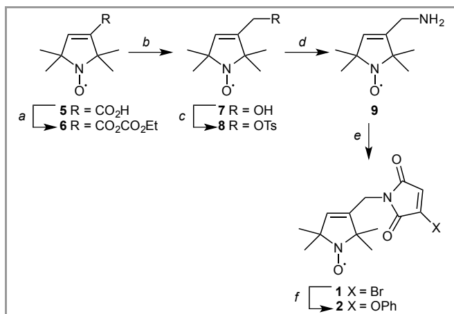
Scheme 2 Reagents and conditions: (a) Ethyl chloroformate, Et 3 N, toluene, quantitative; (b) NaBH 4 , EtOH, 83%; (c) TsCl, Et 3 N, DCM, 67%; (d) NH 3 , MeOH, 80%; (e) Bromomaleic anhydride (1 equiv.), AcOH, 47%; (f) phenol (15 equiv.), t-BuOK (1.2 equiv.), dioxane, 92%.
