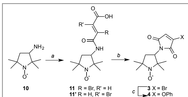
Scheme 3 Reagents and conditions: (a) Bromomaleic anhydride (1 equiv.), ether, 87%; (b) NaOAc (1 equiv.), Ac 2 O, 64%; (c) phenol (15 equiv.), t-BuOK (1.2 equiv.), dioxane, 92%.
