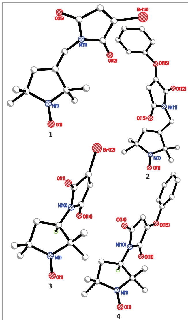
Figure 1 Ball and stick representation of compounds 1 – 4 from X-ray crystallography. The hydrogen atoms are omitted for clarity except for the stereocentre at C3' for 3 and 4. For 3 this representation is from one of three crystallographically independent molecules.
