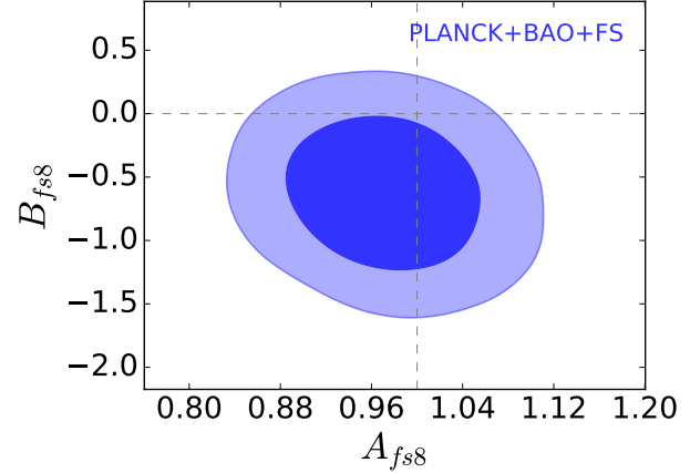
Figure 20. Results for modification of the growth function in the \Lambda CDM cosmological model. The results are consistent with the predictions of General Relativity: A_{f\sigma_8} = 1 , B_{f\sigma_8} = 0 .
