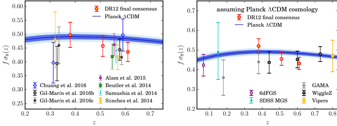
Figure 15. Left-hand panel: Comparison of f\sigma_8(z) measurements across previous BOSS measurements in DR11 (Alam et al. 2015b; Beutler et al. 2014a; Samushia et al. 2014; Sánchez et al. 2014) and DR12 (Gil-Marín et al. 2016b,c; Chuang et al. 2016) samples. The agreement among measurements at better than 1\sigma reflects the fact that many points are obtained from overlapping data sets. Right-hand panel: The f\sigma_8(z) results from this work compared with the measurements of the 2dGRS (Percival et al. 2004b) and 6dFGS (Beutler et al. 2012), the GAMA (Blake et al. 2013), the WiggleZ (Blake et al. 2012), the VVDS (Guzzo et al. 2008), and the VIPERS (de la Torre et al. 2013) surveys, as well as the measurements from the SDSS-I and -II main galaxy sample (Howlett et al. 2015, MGS) and the SDSS-II LRG sample (Oka et al. 2014, DR7). We have plotted conditional constraints on f\sigma_8 assuming a Planck \Lambda CDM background cosmology. This is one of the best evidence of how growth rate measurements from BOSS again reaffirm the validity of General Relativity in large scales.
