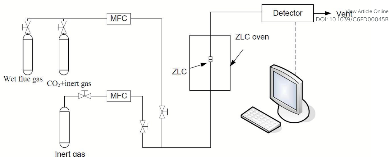
Figure 1: Schematic view of the ZLC apparatus.
