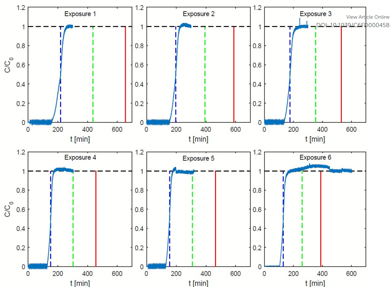
Figure 6: Experimental adsorption curves for H 2 O. Vertical blue, green and red lines indicate first moment, and the times corresponding to 2 and 3 times the first moment respectively.
