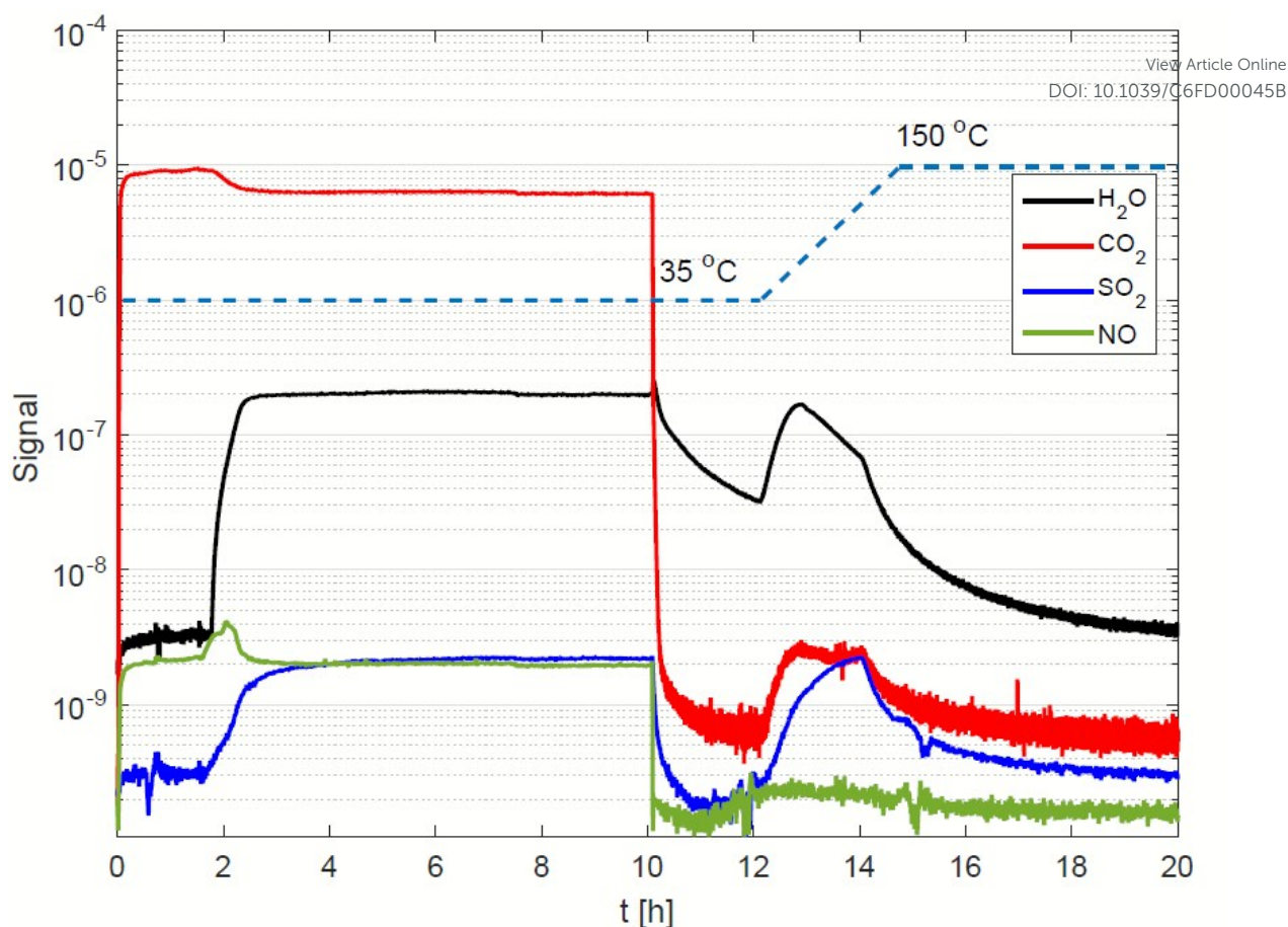
Figure 4: Example of signal acquired during the wet flue gas exposure on the Ni-CPO-27.
