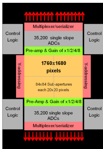
Figure 10: Example of the internal organisation of a highly integrated CMOS sensor for astronomy. The internal architecture is subdivided into separate areas that may be read out in parallel. This particular device is divided into sub apertures 20 x 20 pixels. These may be read out randomly or sequentially. The signals from the sub apertures are pre-amplified and then passed in this device to 70,400 single slope analogue to digital converters. The digitised data are multiplexed to a total of 88 low-voltage differential serial links to be passed back to the computer [25].
