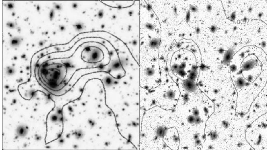
Figure 6: Analysis of the distortion signal to determine the distribution of substructure in the galaxy cluster Abell 1689 using a ground-based wide-field image from Subaru [22] (left) and a deep space-based HST/ACS image (right) [23] with contours showing the reconstructed mass distribution. GravityCam images would be both of high angular resolution and deep (as the space-based data), and at the same time cover a large area like the ground-based data (tens of arc minutes compared to a few arc minutes as HST/ACS).
