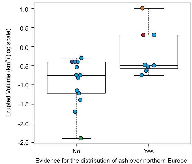
Fig. 7. Boxplots (with overlain jitter plot) showing the total erupted volumes (km 3 ) for the historic silicic eruptions of Icelandic volcanoes (Hekla (light blue), Askja (red), Öraefajökull (orange), Eyjafjallajökull (green) and Torfajökull (dark blue)), n = 21 , volume data compiled by Larsen et al. (1999). Data are grouped into eruptions which resulted in evidence for the distribution of ash over northern Europe, and those for which there is no evidence of ash distribution over northern Europe. Boxplot convention is as follows: boxes indicate the interquartile range; the central line through each box indicates the median. The far extent of the upper and lower lines from each quartile indicate the maximum and minimum. (For interpretation of the references to colour in this figure legend, the reader is referred to the web version of this article.)
