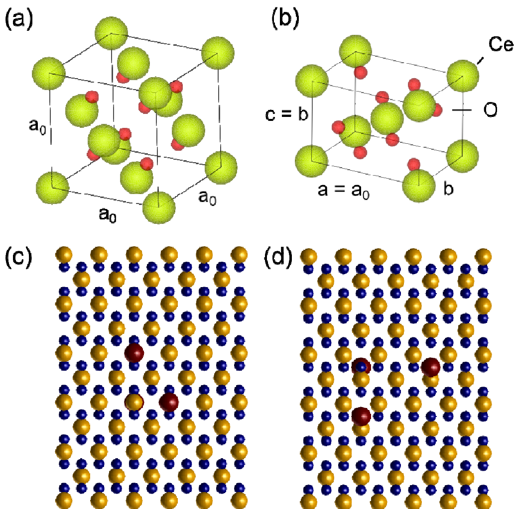
Crystal models showing (a) the \text{CeO}_2 unit cell ( a_0 = 0.541 nm), (b) tetragonal \text{CeO}_2 unit cell with the top representing the [110] \text{CeO}_2 surface ( b = 2^{(-1/2)}a_0 ) and (c) side view of a \text{CeO}_2 supercell showing two possible locations of Au substitutions; and (d) the supercell with the three locations of Au substitutions in Ce vacancies at the surface.
