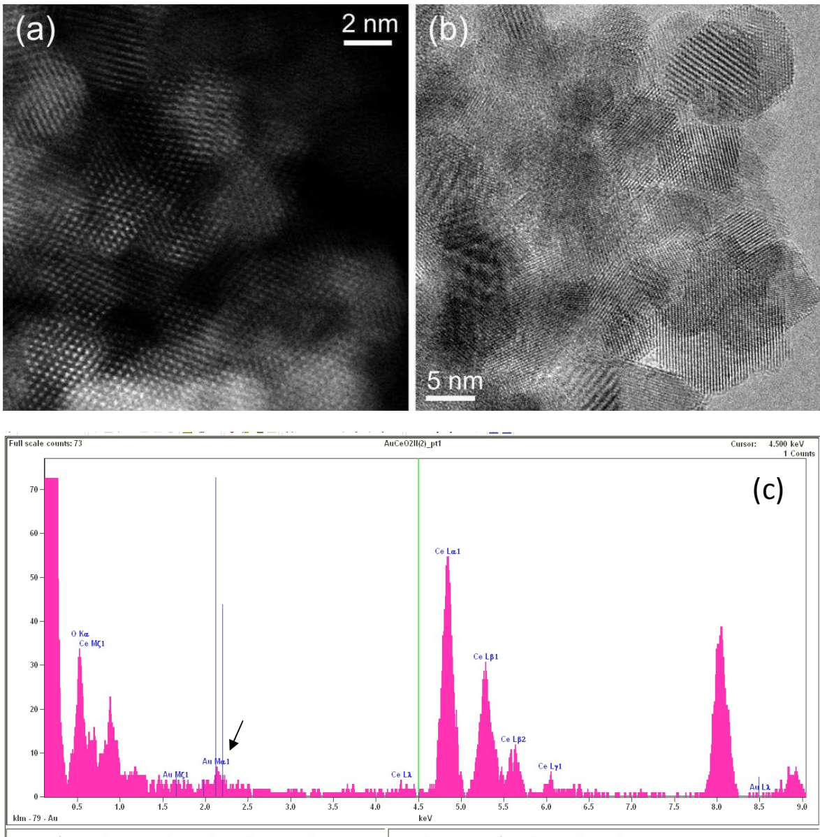
Experimental images of ceria grains in practical catalysts: (a) ESTEM image and (b) ETEM; (c) EDX profile showing the presence of Au in the grains. Ceria grains are primarily in [110] orientations but a few [001] and [112] grains were also observed. Intensity variations in atomic columns in grains of generally uniform thickness are observed in the ESTEM (a). Such variations appear to be common in other similar practical catalysts on ceria supports.
